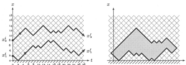
Fig. 1. Two non-intersecting directed walks above a wall (left) and (right) a vesicle made by adding two pairs of steps (grey) to two non-intersecting walks starting and ending a distance two apart.
