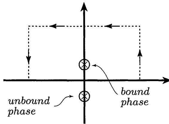
Fig. 2. The contour and pole structure in the complex k -plane, used to evaluate the integral (3.4).
